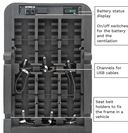
Device frame bottom
