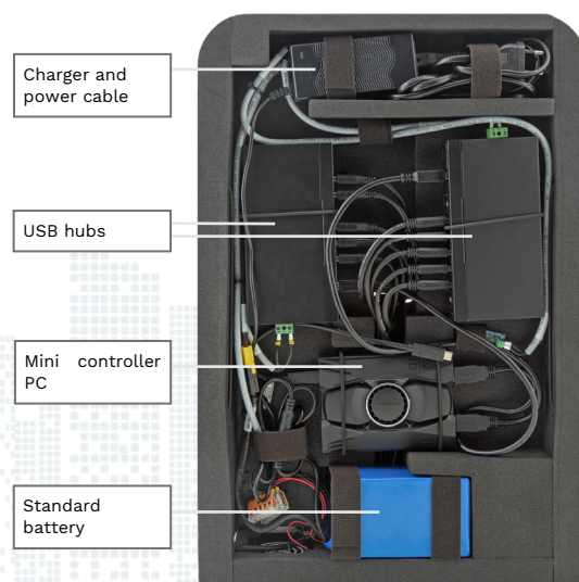
Device frame back
